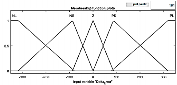
Figure 4. The membership function value of inputs variable "Delta Error".
