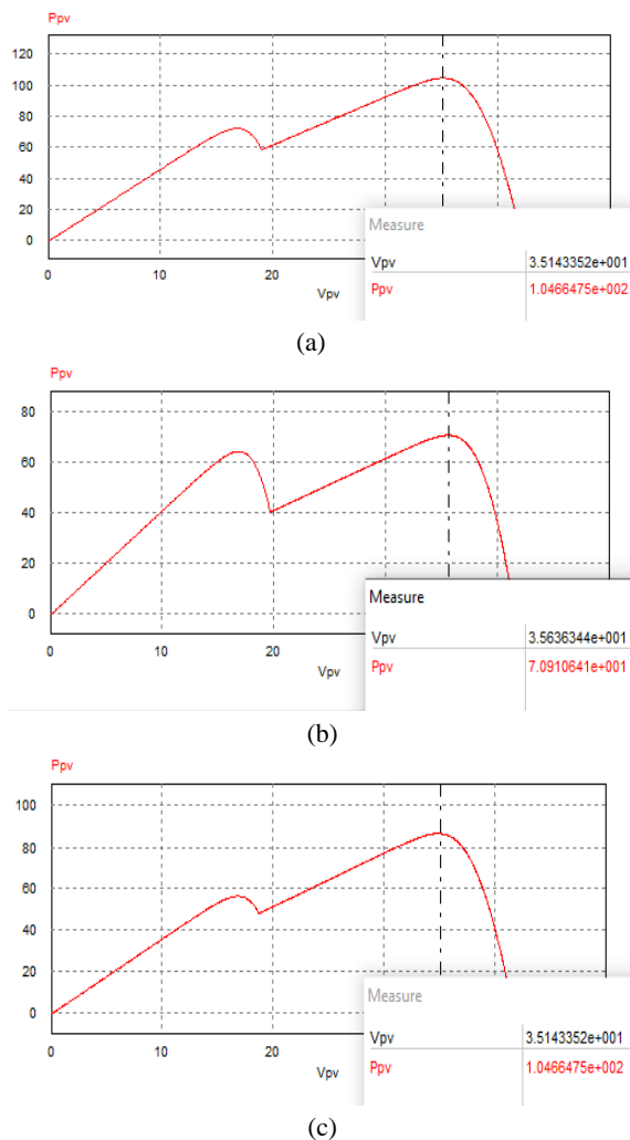
Figure 6. (a), (b) & (c) P-V characteristic curve in partial shading condition.
