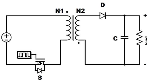
Figure 1. Flyback Converter Circuit
