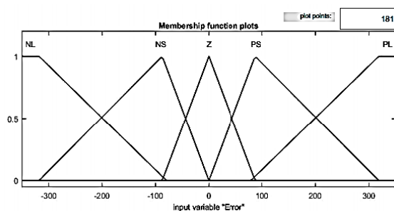
Figure 3. The membership function value of inputs variable "Error"
