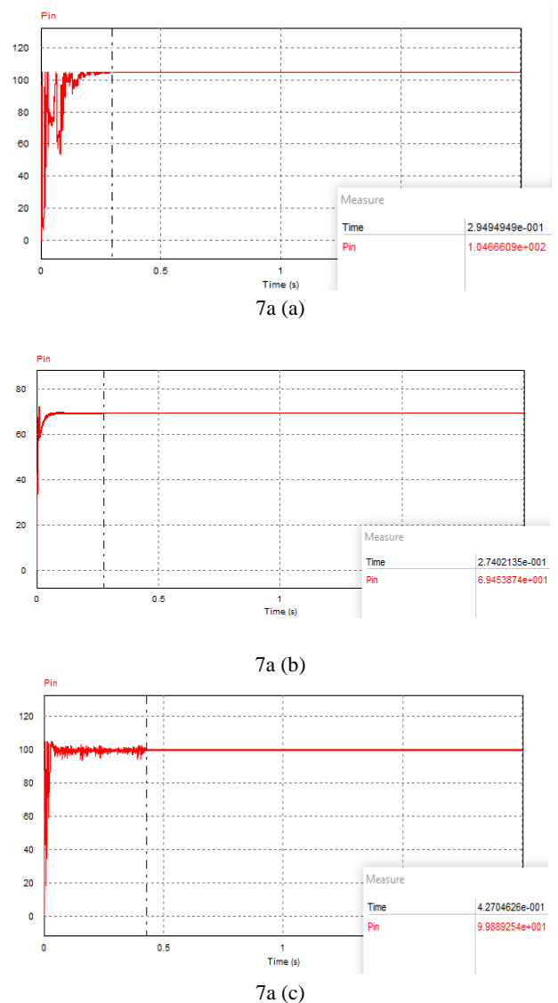
Figure 7a. Result of simulation on pattern 1 (a) HPO, (b) Fuzzy and (c) ABC
