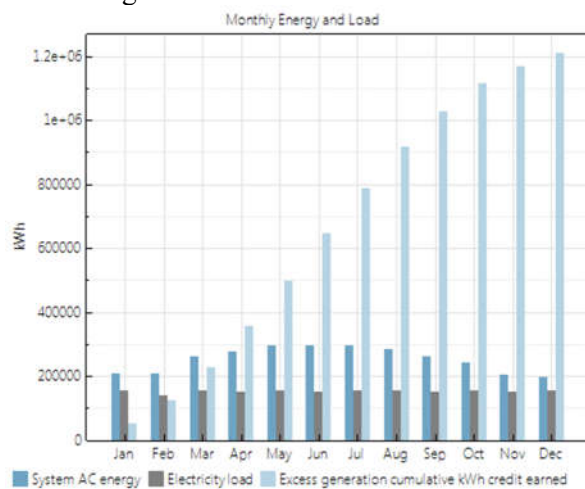
Figure 10. System AC Energy Vs. Load Demand
