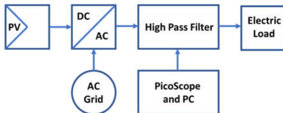
Figure 1. Measurement schematic
